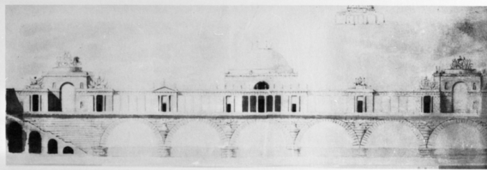
Fig. 4.23. Triumphal bridge design, Parma Academy version, side elevation (SM, Drawer 73).
